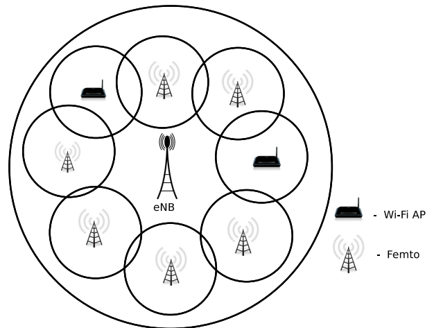
Fig. 1: An example of HetNet comprising of LTE, Wi-Fi, and Femto networks
