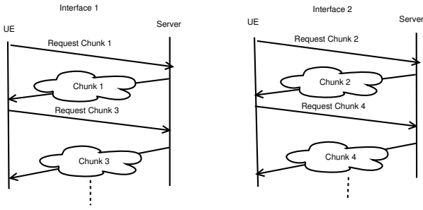
Fig. 3: Example of Request-Response scenario in Sequential DLAS
