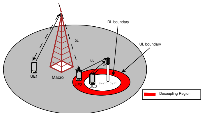
Figure 1. DL/UL Decoupling
